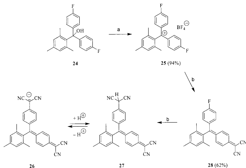
Scheme 5. Twofold \text{S}_\text{N}\text{Ar} reaction with a bis(fluorophenyl)-substituted benzylic cation; a: \text{HBF}_4 -etherate, \text{CH}_2\text{Cl}_2 ; b: malononitrile, NaH, THF.
