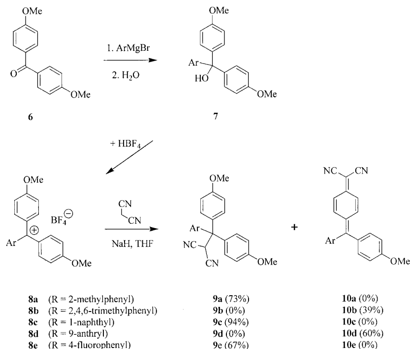
Scheme 2. Dianisyl-substituted benzylic cations: product ratio in relation to steric hindrance.
