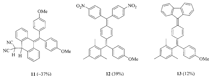
Scheme 3. Additional products from dianisyl-substituted carbocations.
