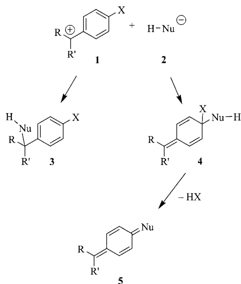
Scheme 1. Reaction pathways for the nucleophilic attack on benzylic cations.
