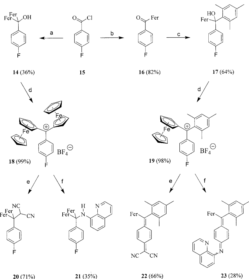
Scheme 4. Test reactions with ferrocenyl-4-fluorophenyl-substituted benzylic cations (Fer = ferrocenyl); a: 3 equiv. ferrocenyl-Li, THF; b: \text{AlCl}_3 , \text{CH}_2\text{Cl}_2 ; c: mesityllithium, THF; d: \text{HBF}_4 -diethyl ether, \text{CH}_2\text{Cl}_2 ; e: malononitrile, NaH, THF; f: 8-aminoquinoline, NaH, THF.
